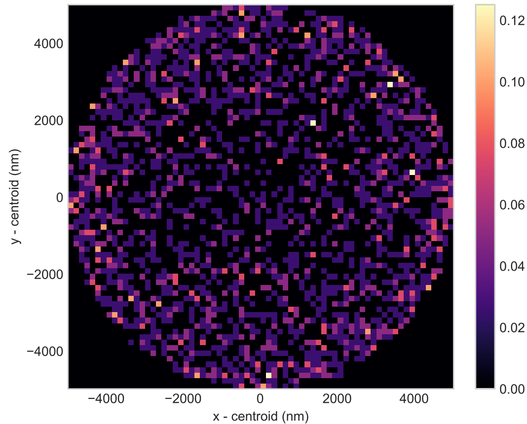
Weighted final ray-density shape
