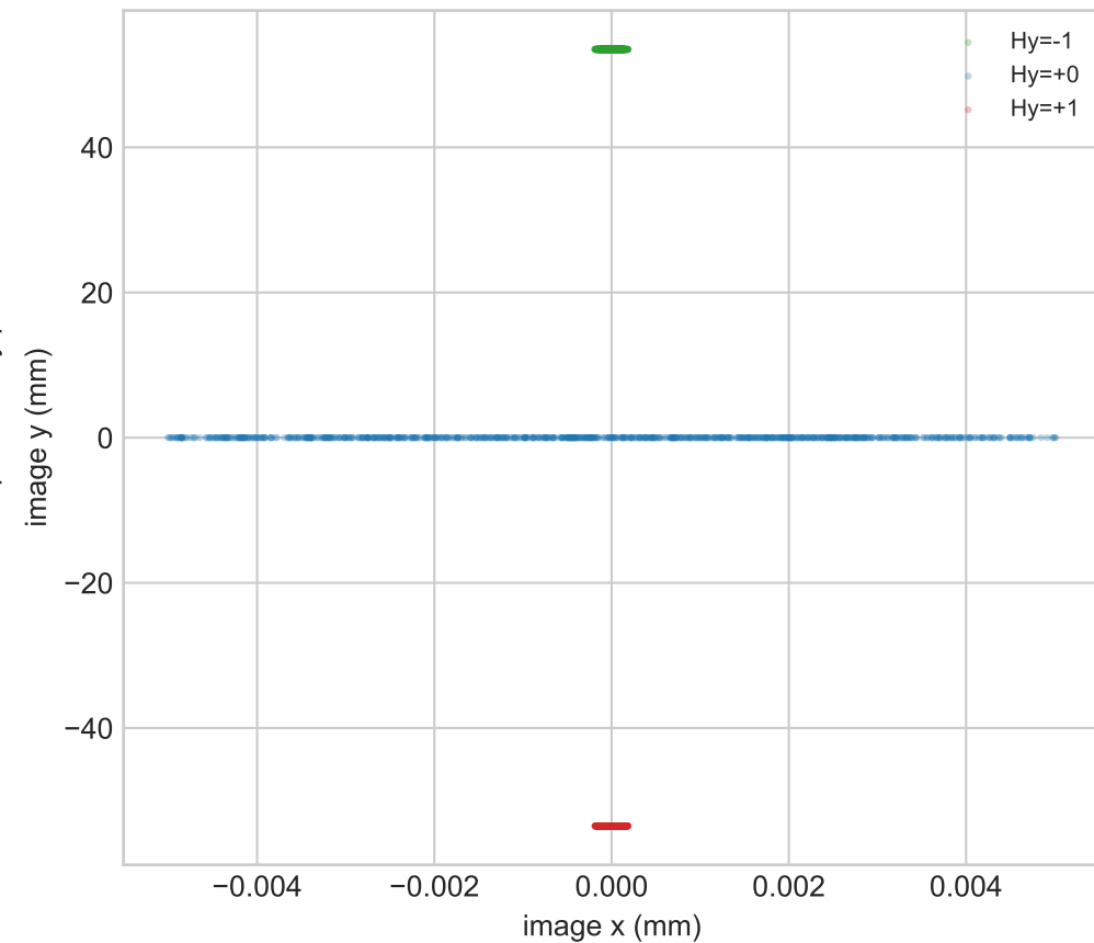
Three ring-field footprints at wafer
