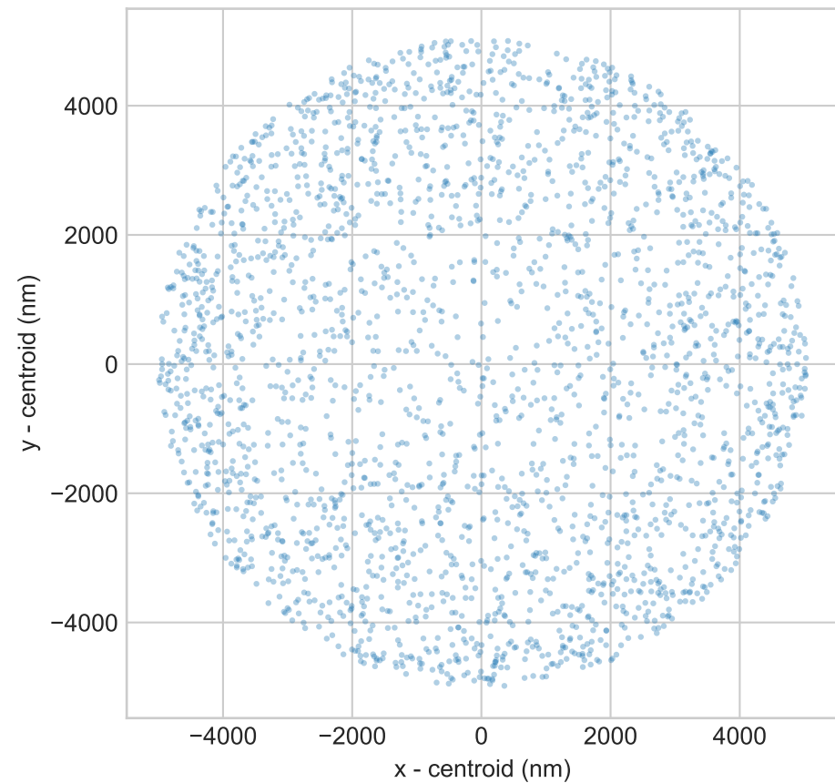
Middle-field spot; RMS radius = 3858.27 nm
